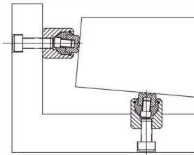
Gripper Swivel Pads can be surface mounted or installed in a counterbored hole.
